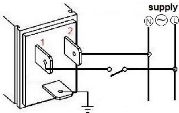
Figure 3 – Connection diagram for alternating voltage
