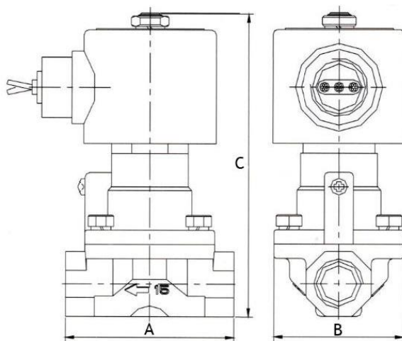
Figure 2 - Valve dimensions DN15-50
