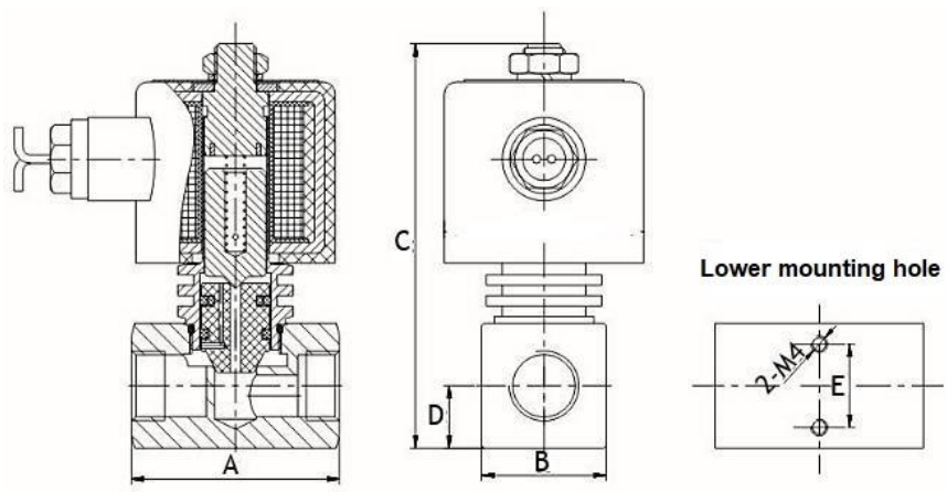
Figure 1 - Valve dimensions DN8-10
